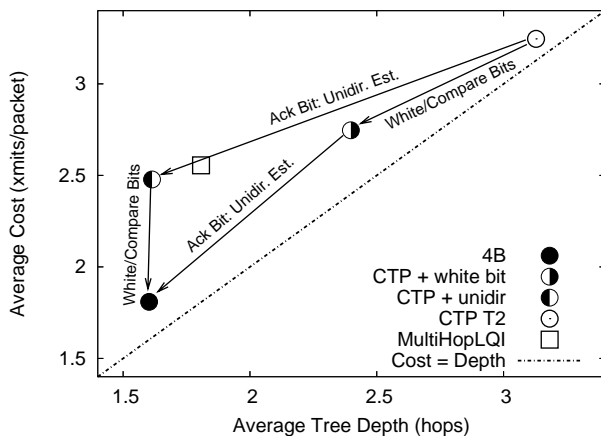
Figure 6. Exploring the link estimation design space: adding the ack bit and/or the white and compare bits to CTP decreases cost (lower is better) and the average depth of a node in the routing tree.
