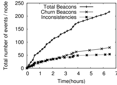
(b) Control overhead from route inconsistencies.
