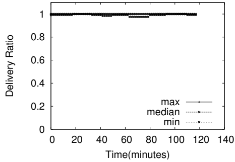
(a) Nodes fail at 60 minutes and CTP does not observe any significant disruption.
