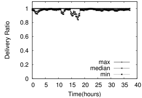
(a) Delivery Ratio for CTP
